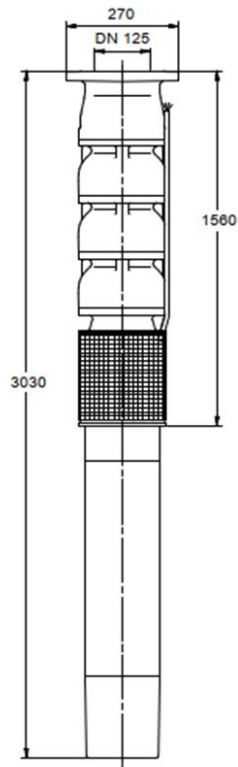
Figure 2 A detail of the adopted submersible pump
